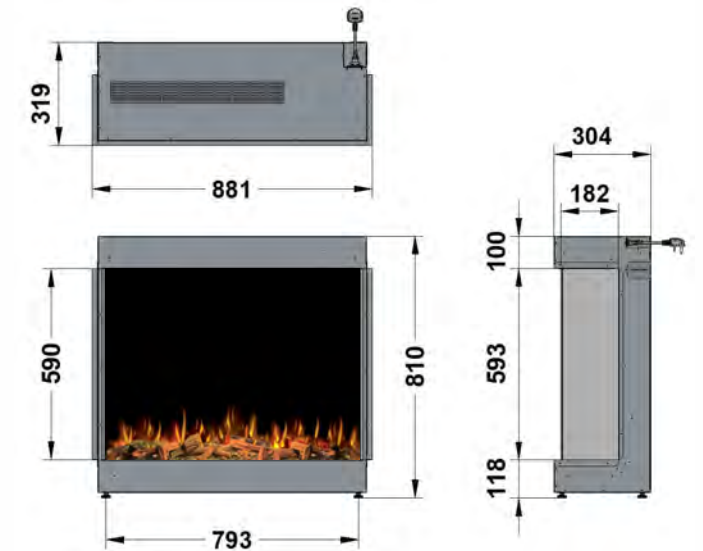
950 ASPECT - BAY
