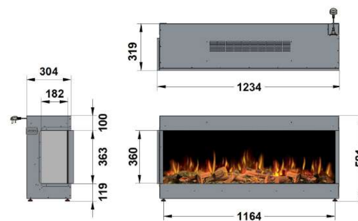
1250 - LEFT CORNER
